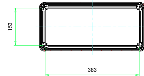
C-C (1:6.5)
